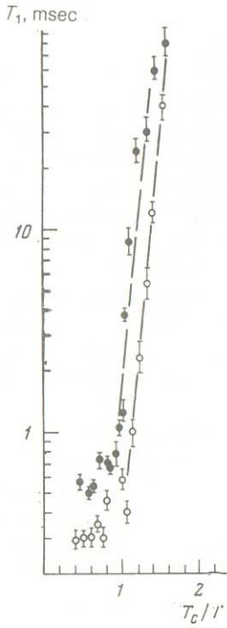
FIG. 8. Temperature dependence of the spin-lattice relaxation time of ^{63}\text{Cu} in the Cu(2) for the compound \text{YBa}_2\text{Cu}_3\text{O}_{6.95} : \circ —unirradiated sample, T_c = 93 K; \bullet —sample irradiated by a fluence \Phi = 5 \cdot 10^{18} \text{ cm}^{-2} , T_c = 71 K.
