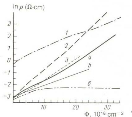
FIG. 5. Dependence of \ln \rho on fluence \Phi obtained in the process of irradiation at T = 80 \text{ K} : 1— \text{La}_2\text{CuO}_4 , 2— \text{YBa}_2\text{Cu}_3\text{O}_{6.95} , 3—single-crystal Y-Ba-Cu-O, \rho measured perpendicular to the c -axis, 4— \text{La}_{1.83}\text{Sr}_{0.17}\text{CuO}_4 , 5—Bi-Sr-Ca-Cu-O, 6— \text{SnMo}_6\text{S}_8 .
