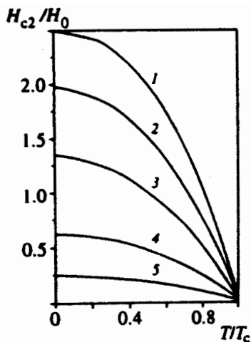
FIG. 11. The temperature behavior of the upper critical field for systems with different degrees of disorder \gamma/T_{c0} . The pairing coupling constant g=2 , the magnetic field is in units of H_0 = (2/\pi)\phi_0 T_{c0}/v_F^2 and the temperature is normalized to T_c , which is disorder-dependent. Curve 1, \gamma/T_{c0}=0.2 ; curve 2, \gamma/T_{c0}=0.25 ; curve 3, \gamma/T_{c0}=0.5 ; curve 4, \gamma/T_{c0}=0.75 ; and curve 5, \gamma/T_{c0}=0.87 .
