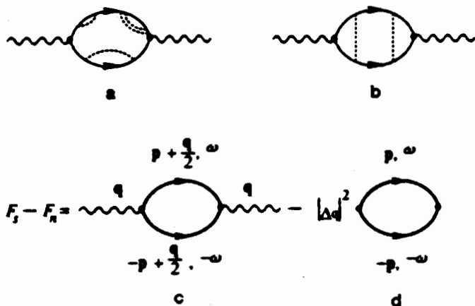
FIG. 6. Diagrammatic expansion of the free energy in the presence of impurity scattering. The dashed lines correspond to scattering by impurities.
