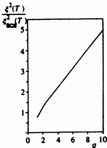
FIG. 3. The dimensionless coherence length as a function of the coupling constant g .
