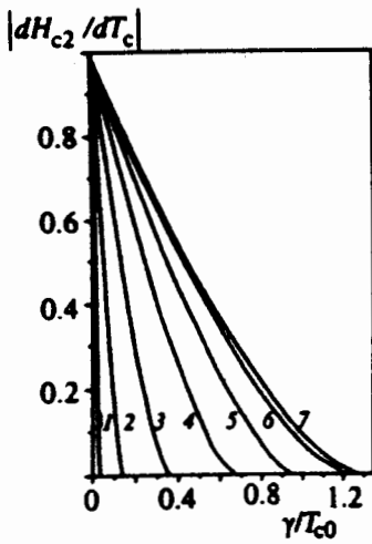
FIG. 9. The slope of the upper critical field H_{c2} vs impurity scattering rate curve for different values of the coupling constant g : curve 1, g=1.22 ; curve 2, g=1.24 ; curve 3, g=1.3 ; curve 4, g=1.5 ; curve 5, g=2.0 ; curve 6, g=5.0 ; and curve 7, g=10.0 . The field's derivative is normalized to its value in the absence of scattering.
