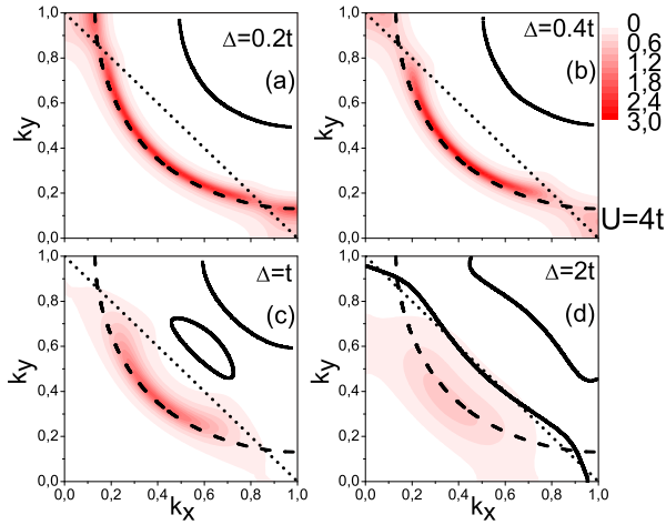
Fig.2. “Destruction” of the Fermi surface as obtained from the DMFT+ \Sigma_{\mathbf{k}} calculations for U = 4t and n = 0.8 . Notations are the same as used in Fig. 1. (a) – \Delta = 0.2t ; (b) – \Delta = 0.4t ; (c) – \Delta = t ; (d) – \Delta = 2t . Black lines show the solution of Eq. (15).
