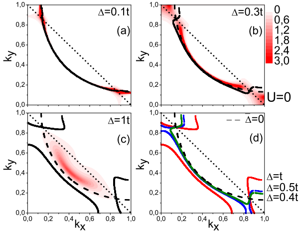
Fig.1. Fermi surfaces obtained for uncorrelated case of U = 0 and filling factor n = 0.8 . Shown are intensity plots of spectral density (14) for \omega = 0 . (a) – \Delta = 0.1t ; (b) – \Delta = 0.3t ; (c) – \Delta = t ; (d) – “Fermi surfaces” obtained solving Eq. (15). Dashed line denotes “bare” Fermi surface.
